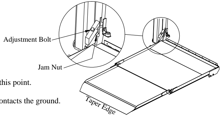
Figure 19: Unfolded 650 platform.
